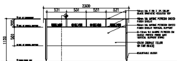
WRITING DECK FRONT ELEVATION SCALE: 1:30 METERS
