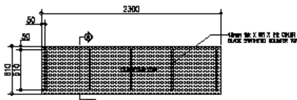
WRITING DECK COUNTERTOP PLAN SCALE: 1:30 METERS
